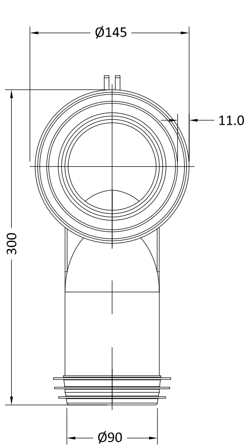
TOP VIEW
