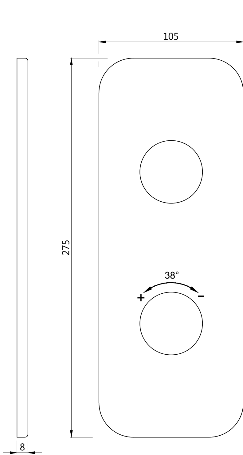
WALL FLANGE
