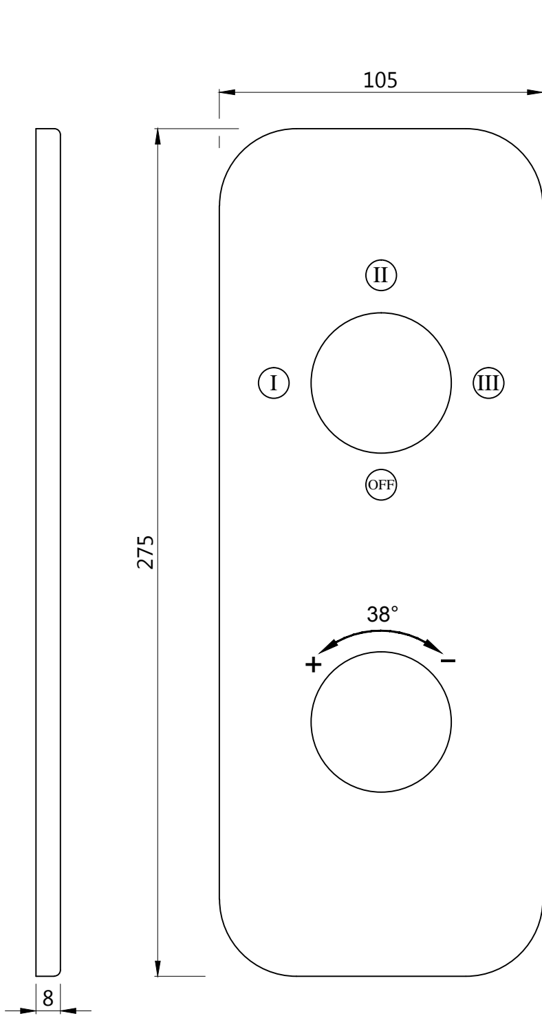
WALL FLANGE
