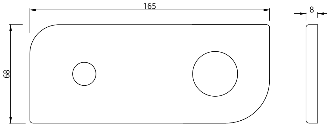
WALL FLANGE
