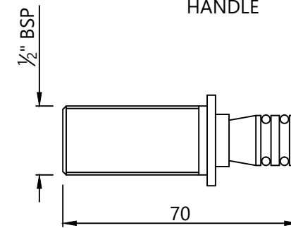
SPOUT NIPPLE
