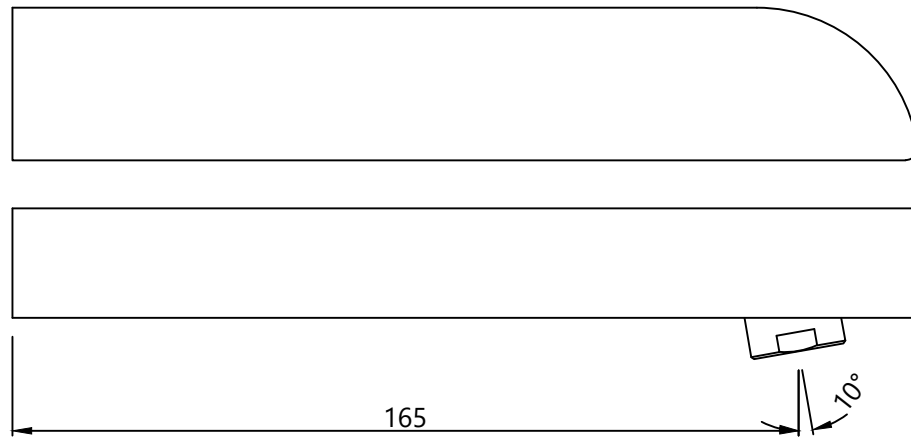
SPOUT
