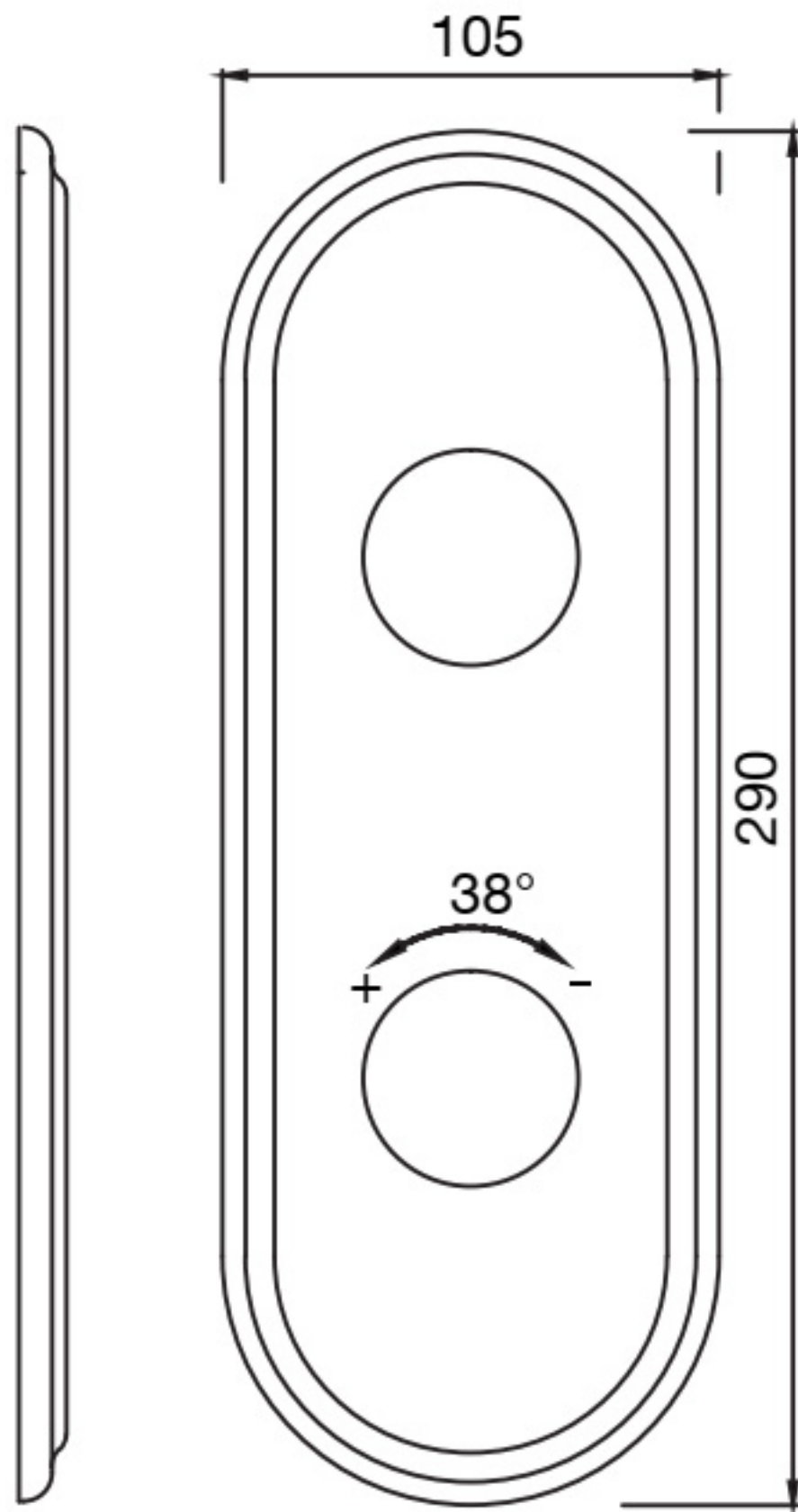
WALL FLANGE
