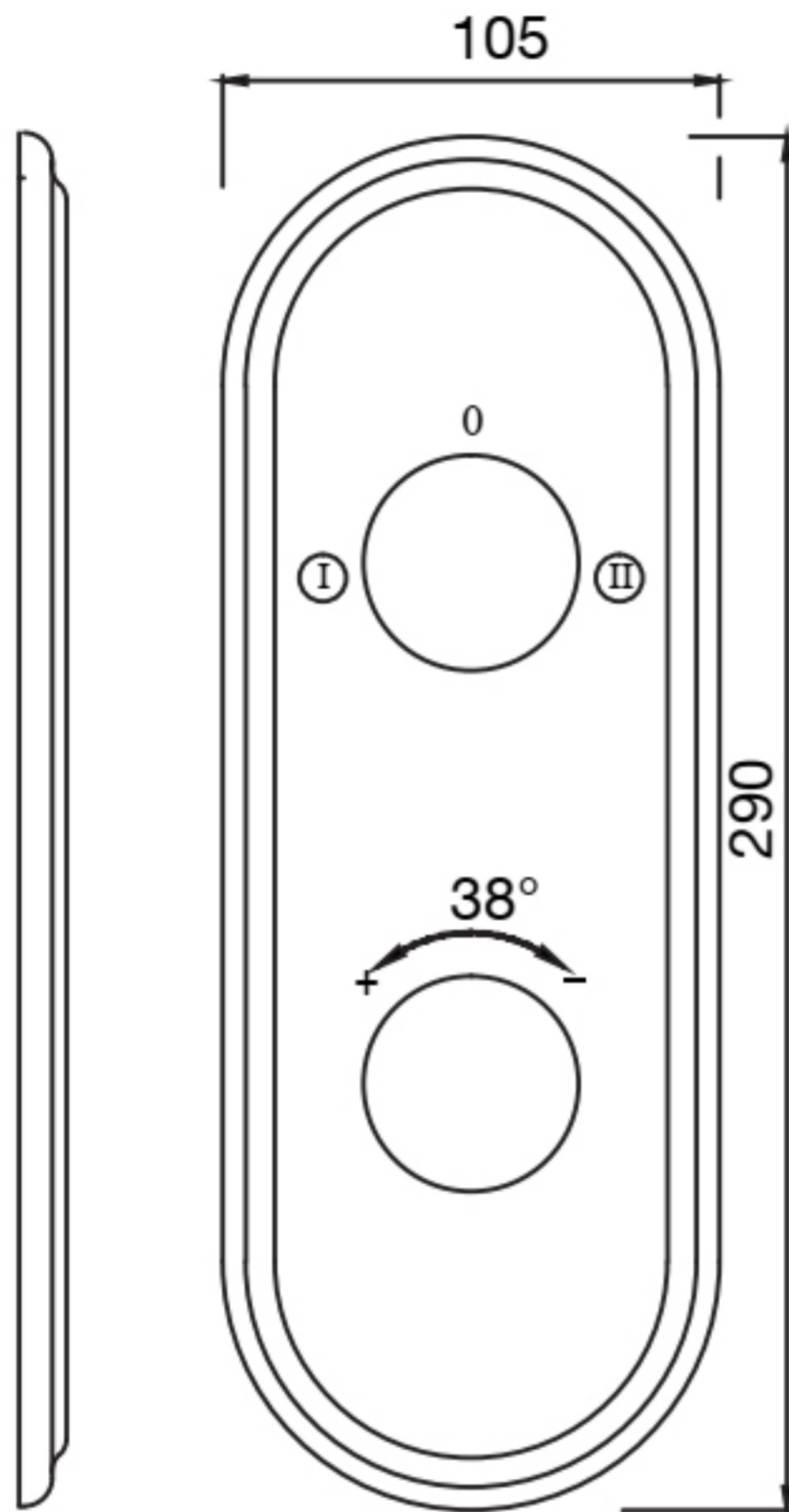
WALL FLANGE
